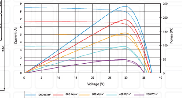
Current-Voltage & Power-Voltage Curve (SV220-20M)
