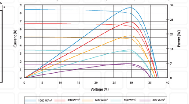
Current-Voltage & Power-Voltage Curve (SV030-12M)
