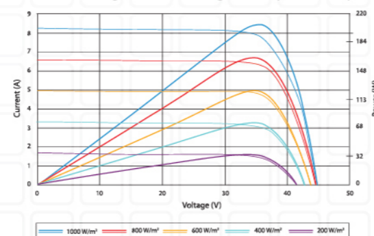
Current-Voltage & Power-Voltage Curve (SV200-18P)
