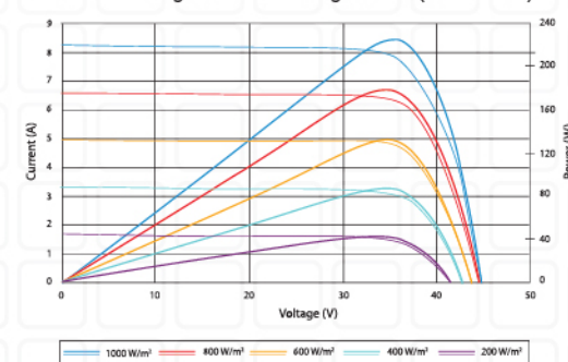
Current-Voltage & Power-Voltage Curve (SV220-20P)
