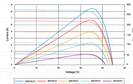
Current-Voltage & Power-Voltage Curve (SV280-24M)
