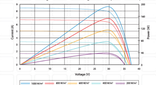
Current Voltage & Power Voltage Curve (SV160 20M)
