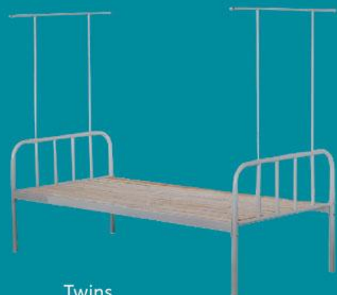
Twins Model: PV-705N Size: L2000*W900*H750mm
